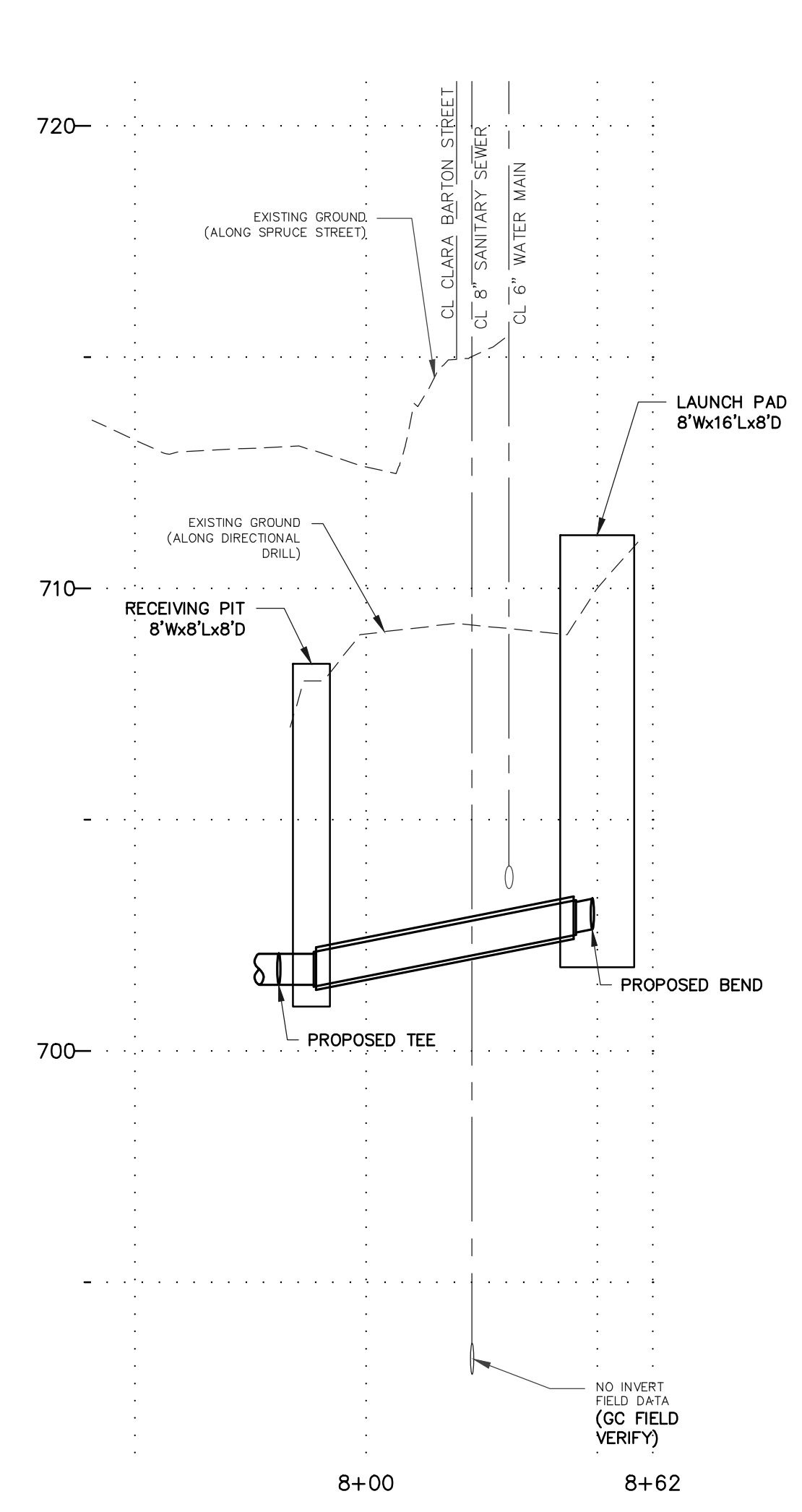
CENTERLINE SPRUCE AVENUE HORIZ SCALE: 1" = 30' VERT SCALE: 1" = 3' (DIR. DRILL UNDER CLARA BARTON)
